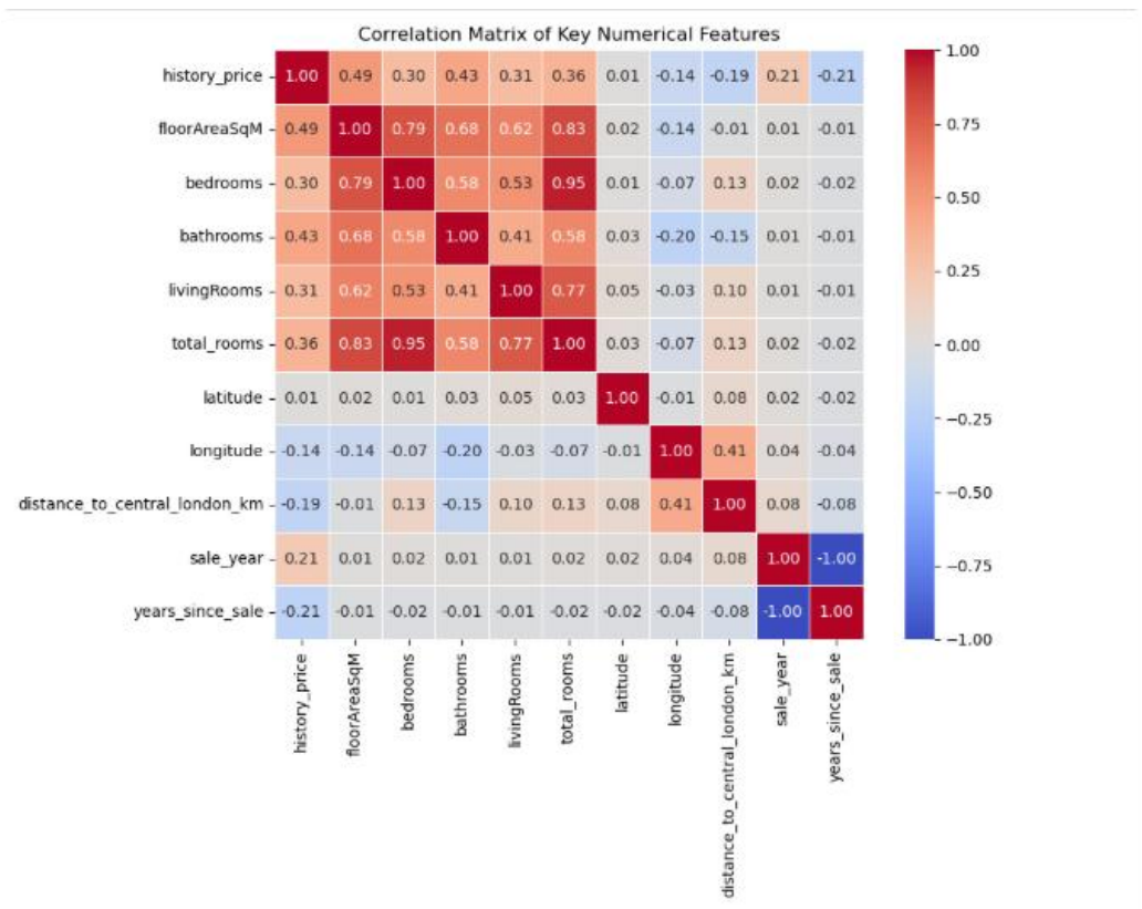
Figure 6: Correlation matrix of key numerical features.
